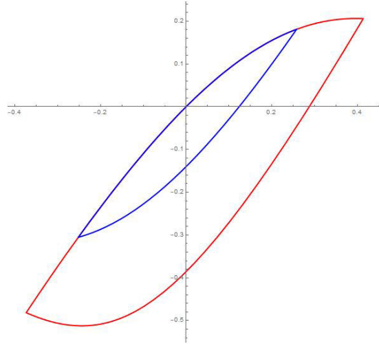
Рис. 2: System trajectories
