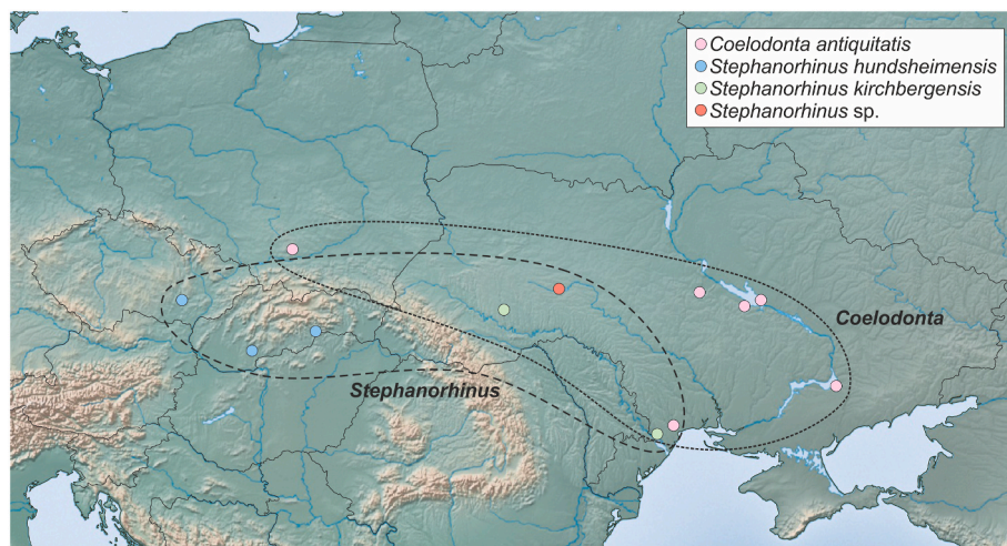
Fig. 2. Distribution of localities yielding rhino remains dated from the late Early Pleistocene to the Middle Pleistocene (MIS 19 – MIS 9) in Central and Eastern Europe.
