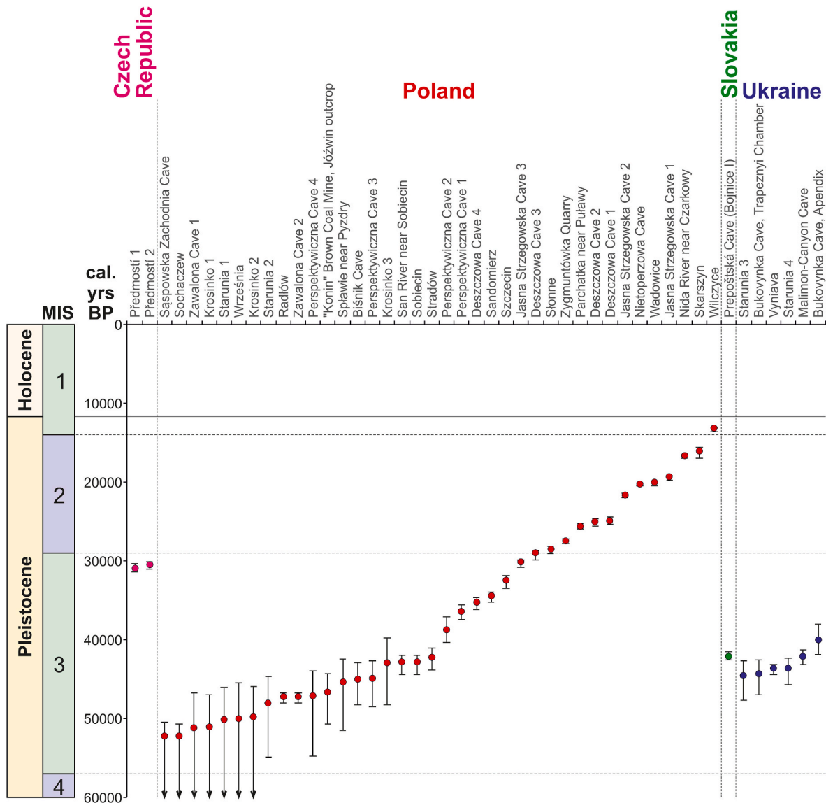
Fig. 9. Distribution of directly dated woolly rhinoceros remains in Central and Eastern Europe during Marine Oxygen Isotope Stage 2–4 (MIS 2–4).
