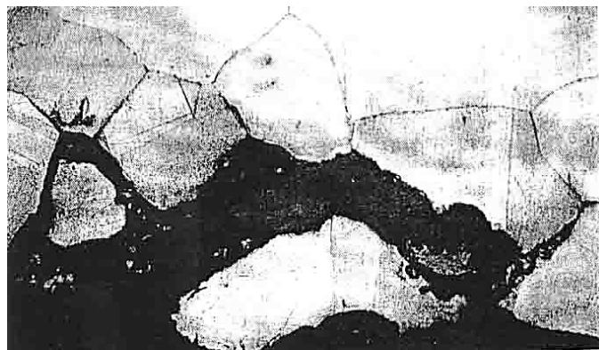
Fig. 1. Cracking of the cathode material in the near-surface layer.
