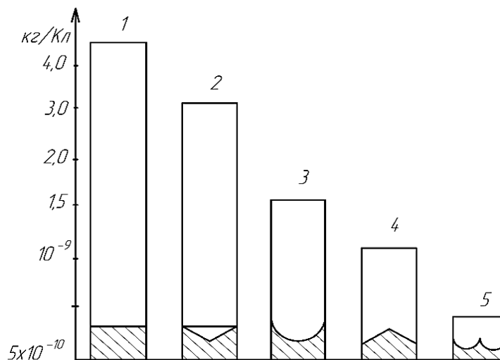
Fig. 2. The magnitude of specific erosion for different geometry of the bottom of the copper electrode.
