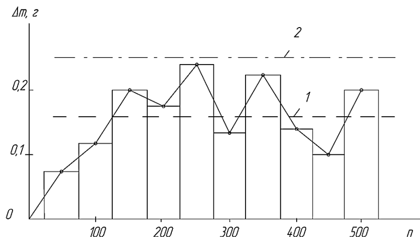
Fig. 3. Wear of a copper electrode at different operating currents, A: 1 – 180; 2 – 350.
