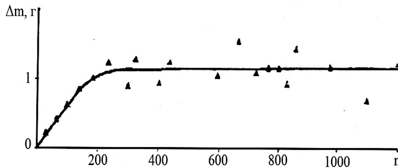
Fig. 4. Change in wear rate of copper electrode.
